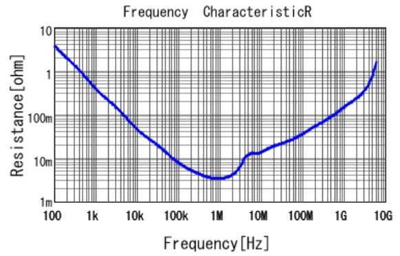
■ GRM188D71A106MA73 R DCOV, 25degC
