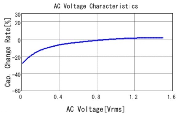
■ GRM188D71A106MA73 C-AC Voltage capchange, DCOV, 25.0d
