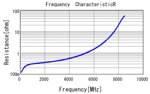
■ GRM1885C1H6R9WA01 R DCOV, 25degC
