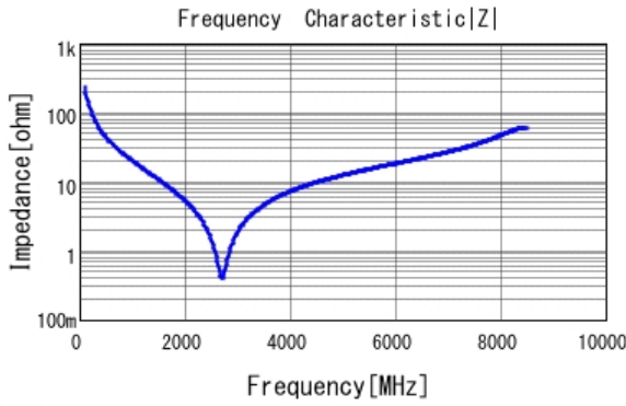
■ GRM1885C1H6R9WA01 |Z| DCOV, 25degC
