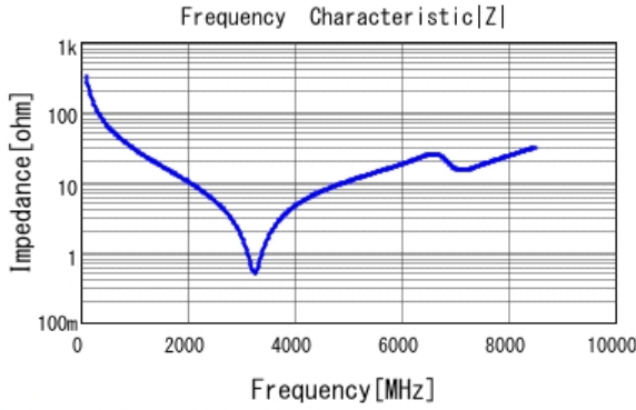
■ GRM1885C1H4R9BA01 |Z| DCOV, 25degC
