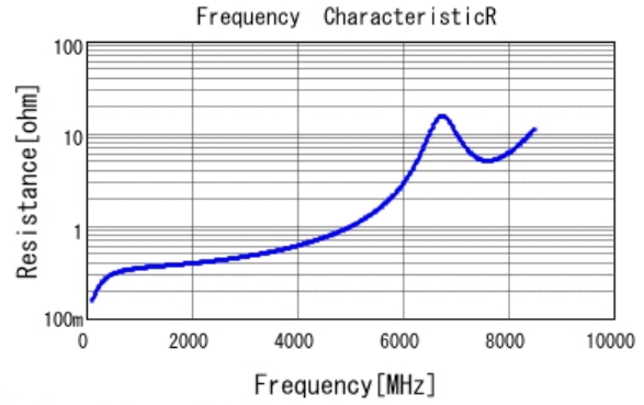
■ GRM1885C1H4R9BA01 R DCOV, 25degC
