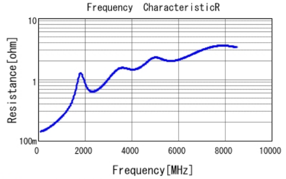
■ GRM1885C1H680JA01 R DCOV, 25degC
