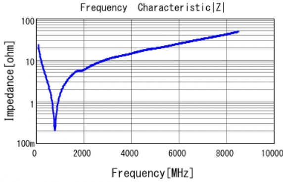
■ GRM1885C1H680JA01 |Z| DCOV, 25degC
