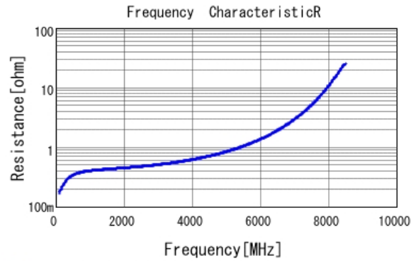
■ GRM1885C1H2R8CA01 R DCOV, 25degC
