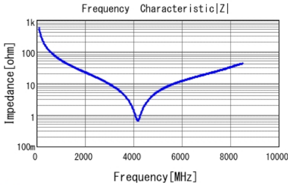
■ GRM1885C1H2R8CA01 |Z| DCOV, 25degC
