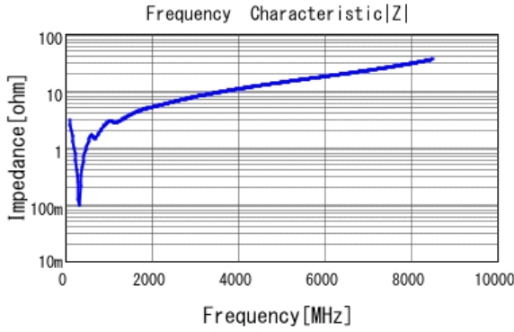
■ GRM1885C1H471JA01 |Z| DCOV, 25degC
