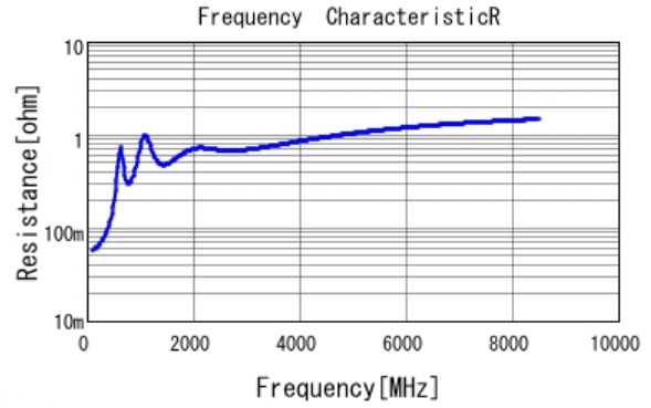
■ GRM1885C1H471JA01 R DCOV, 25degC
