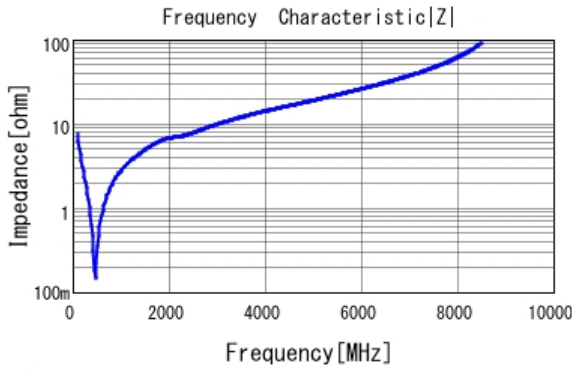
■ GRM1885C1H201JA01 |Z| DCOV, 25degC
