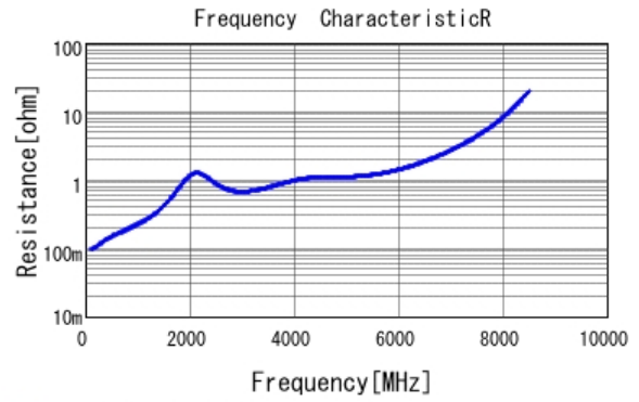
■ GRM1885C1H201JA01 R DCOV, 25degC
