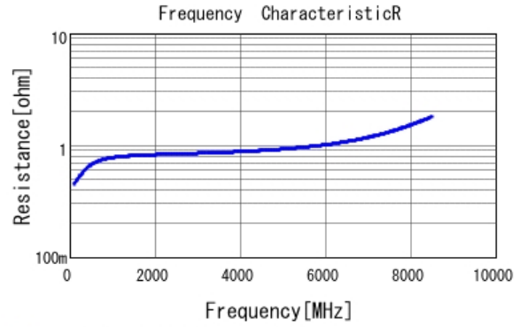
■ GRM1884C1HR70BA01 R DCOV, 20degC
