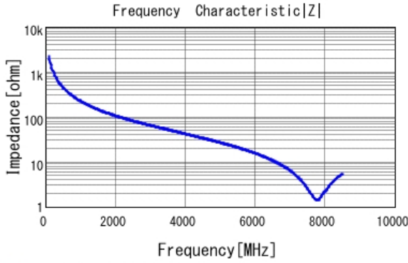
■ GRM1884C1HR70BA01 |Z| DCOV, 20degC
