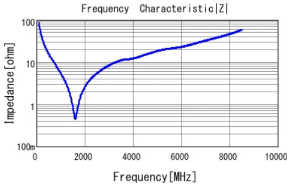
■ GRM1885C1H180JA01 |Z| DCOV, 25degC
