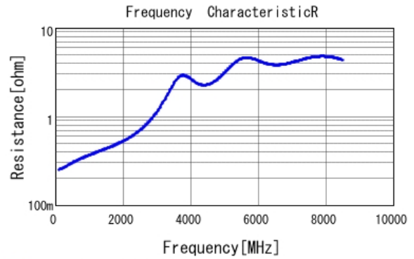
■ GRM1885C1H180JA01 R DCOV, 25degC
