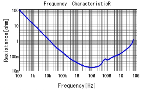
■ GRM155R71C104KA88 R DCOV, 25degC
