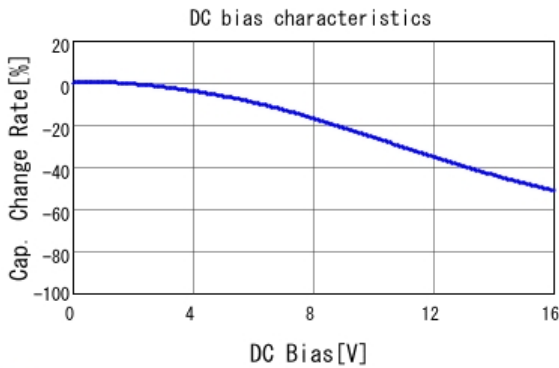
■ GRM155R71C104KA88 C-DC bias capchange, 25.0degC, AC1.
