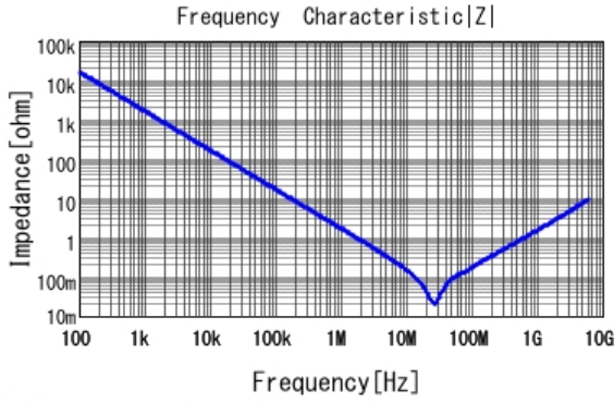
■ GRM155R71C104KA88 |Z| DCOV, 25degC
