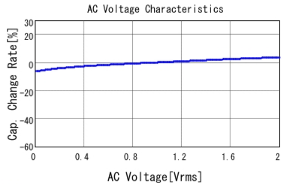
■ GRM155R71C104KA88 C-AC Voltage capchange, DCOV, 25.0d
