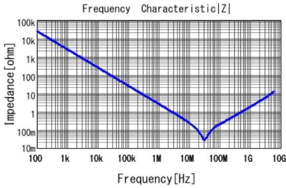
■ GRM155R61A683KA01 |Z| DCOV, 25degC
