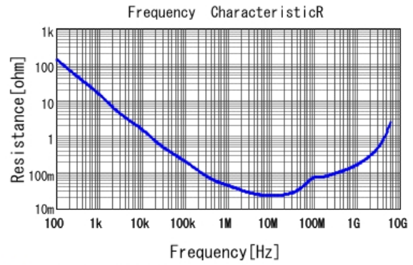
■ GRM155R61A683KA01 R DCOV, 25degC
