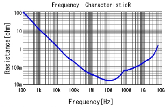
■ GRM155R61A104KA01 R DCOV, 25degC
