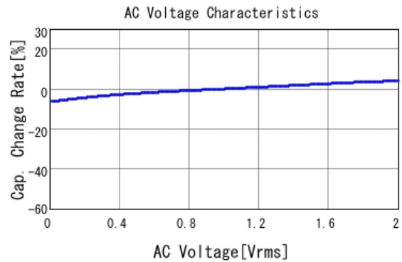
■ GRM155R61A104KA01 C-AC Voltage capchange, DCOV, 25.0d
