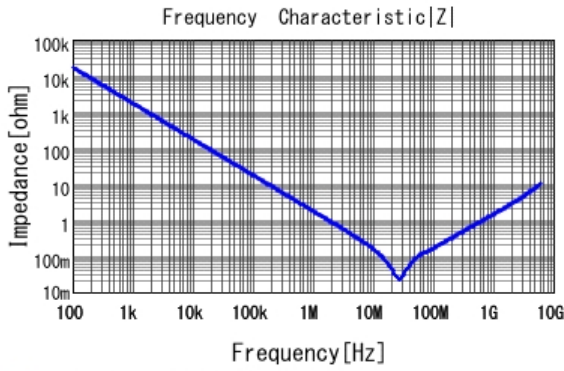
■ GRM155R61A104KA01 |Z| DCOV, 25degC
