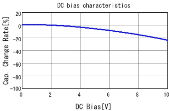
■ GRM155R61A104KA01 C-DC bias capchange, 25.0degC, AC1.
