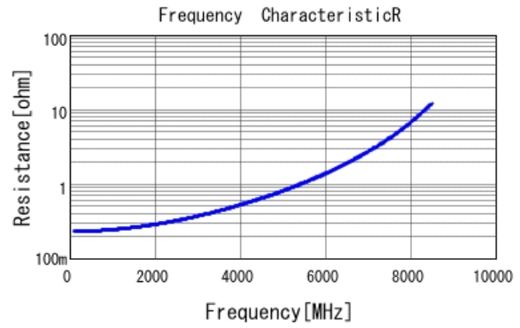
■ GRM1555C1H3R9CA01 R DCOV, 25degC
