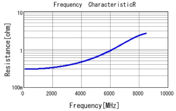
■ GRM1555C1H2R7CA01 R DCOV, 25degC
