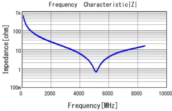
■ GRM1555C1H2R7CA01 |Z| DCOV, 25degC
