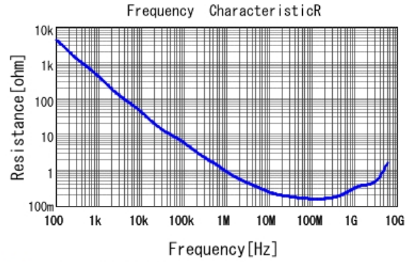
■ GRM033R71A222KA01 R DCOV, 25degC
