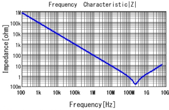
■ GRM033R71A222KA01 |Z| DCOV, 25degC
