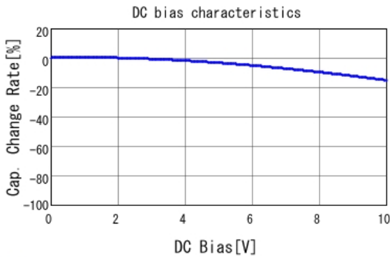
■ GRM033R71A222KA01 C-DC bias capchange, 25.0degC, AC1.
