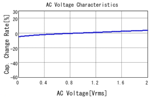
■ GRM033R71A222KA01 C-AC Voltage capchange, DCOV, 25.0d
