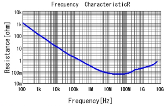
■ GRM033R61A103KA01 R DCOV, 25degC
