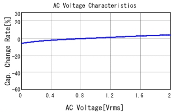
■ GRM033R61A103KA01 C-AC Voltage capchange, DCOV, 25.0d
