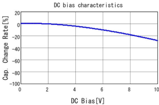
■ GRM033R61A103KA01 C-DC bias capchange, 25.0degC, AC1.
