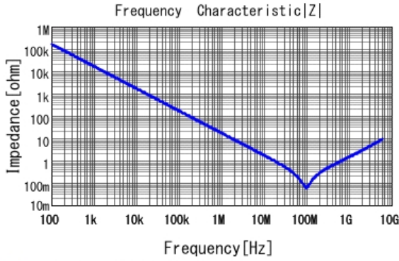
■ GRM033R61A103KA01 |Z| DCOV, 25degC
