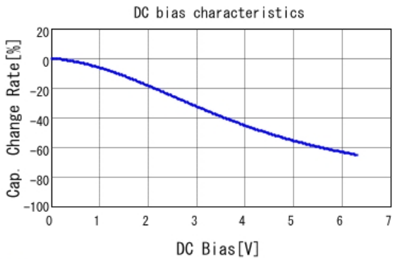
■ GRM033R60J104KE19 C-DC bias capchange, 25.0degC, AC0.
