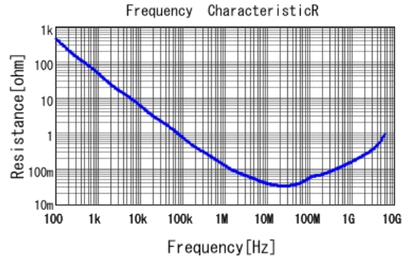
■ GRM033R60J104KE19 R DCOV, 25degC
