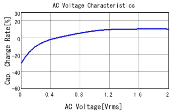
■ GRM033R60J104KE19 C-AC Voltage capchange, DCOV, 25.0d
