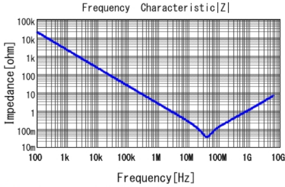
■ GRM033R60J104KE19 |Z| DCOV, 25degC
