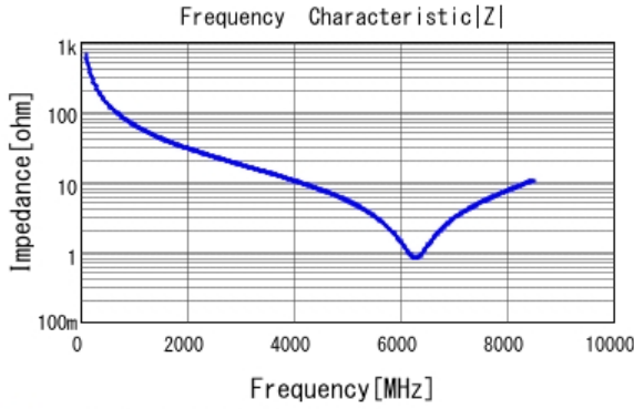
■ GRM0335C1H2R4BA01 |Z| DCOV, 25degC
