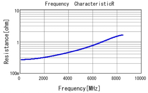
■ GRM0335C1H2R4BA01 R DCOV, 25degC
