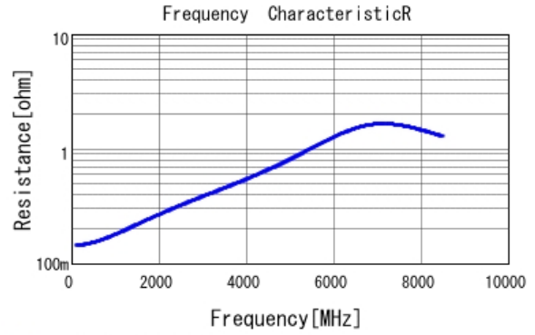
■ GRM0335C1H300JA01 R DCOV, 25degC
