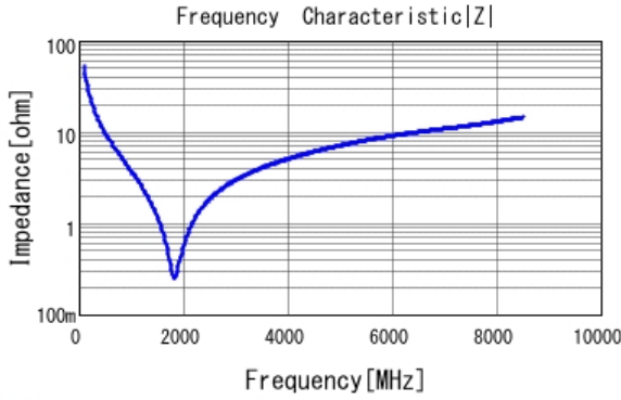
■ GRM0335C1H300JA01 |Z| DCOV, 25degC
