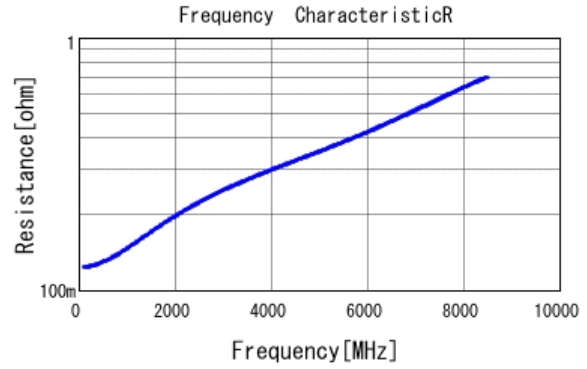
■ GRM0115C1E8R7DE01 R DCOV, 25degC
