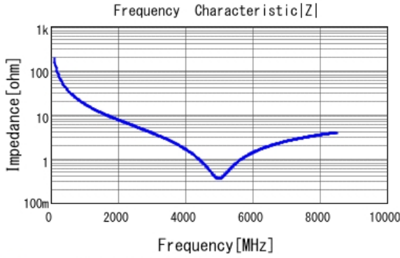
■ GRM0115C1E8R7DE01 |Z| DCOV, 25degC
