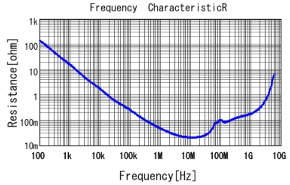
GCM188R71H473KA55 R DCOV, 25degC
