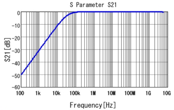
■ GCM188R71H473KA55 S21 DC0V, 25degC
