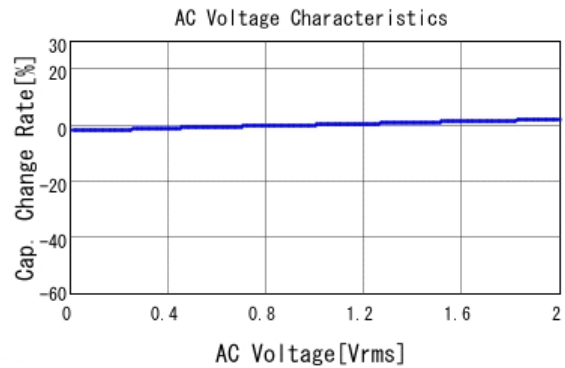
GCM188R71H473KA55 C-AC Voltage capchange, DCOV, 25.0d
