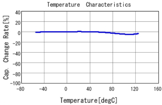
■ GCM188R71H473KA55 C-Temp. capchange, DC0.0V, AC1.0Vrm
