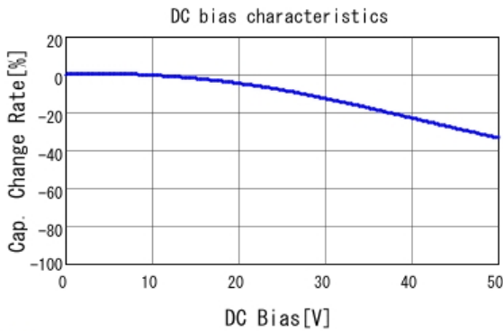
GCM188R71H473KA55 C-DC bias capchange, 25.0degC, AC1.
