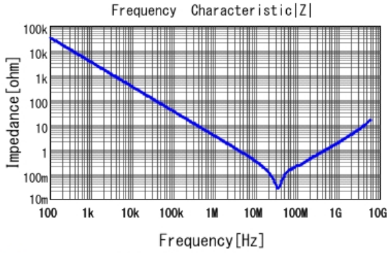
GCM188R71H473KA55 |Z| DCOV, 25degC
