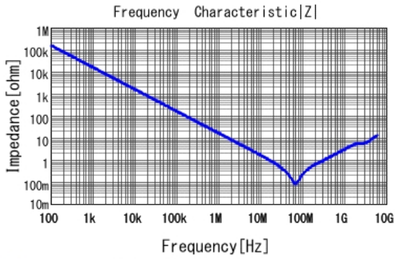
GCM188R71H103KA37 |Z| DCOV, 25degC
