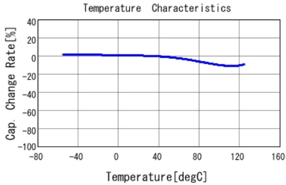
■ GCM188R71H103KA37 C-Temp. capchange, DC0.0V, AC1.0V rm
