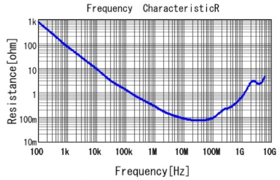
GCM188R71H103KA37 R DCOV, 25degC
