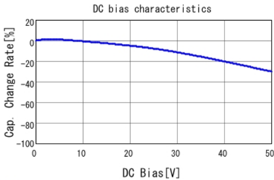
GCM188R71H103KA37 C-DC bias capchange, 25.0degC, AC1.
