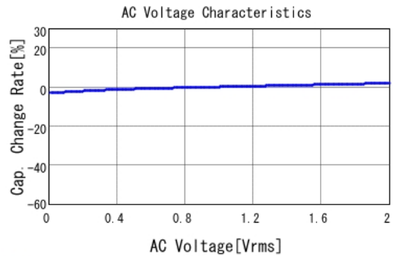
GCM188R71H103KA37 C-AC Voltage capchange, DCOV, 25.0d
