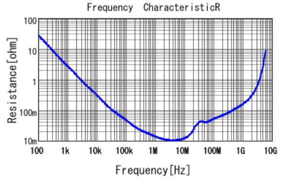
■ GCM188R71C334KA37 R DCOV, 25degC
