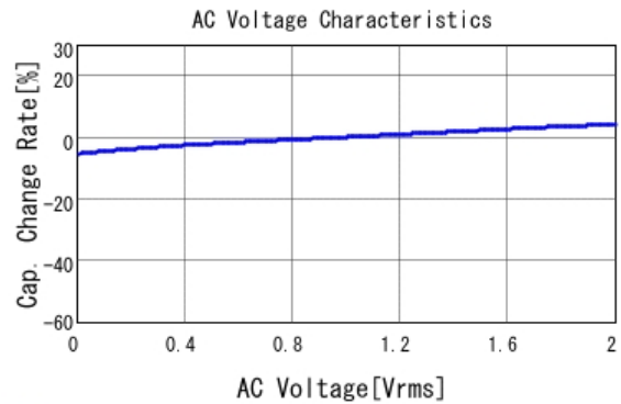
■ GCM188R71C334KA37 C-AC Voltage capchange, DCOV, 25.0d
