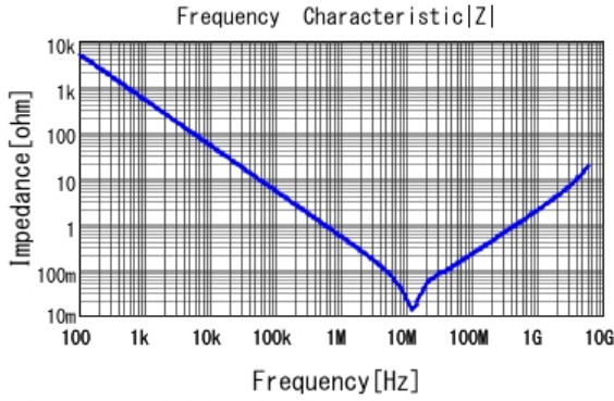
■ GCM188R71C334KA37 |Z| DCOV, 25degC
