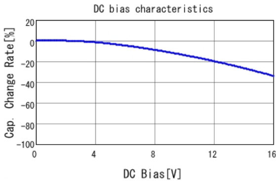
■ GCM188R71C334KA37 C-DC bias capchange, 25.0degC, AC1.
