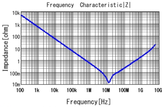
GCM188R71C334KA37 |Z| DCOV, 25degC
