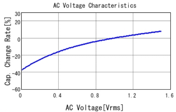
■ GCJ31CR71C106KA15 C-AC Voltage capchange, DCOV, 25.0d
