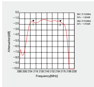
In-band Characteristic
