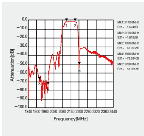
Pass-band Characteristic
