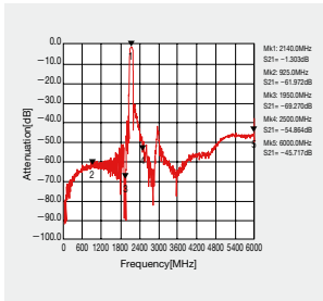
Wide-band Characteristic
