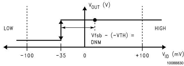
FIGURE 6. VTC of the DS90LV048A LVDS Receiver
