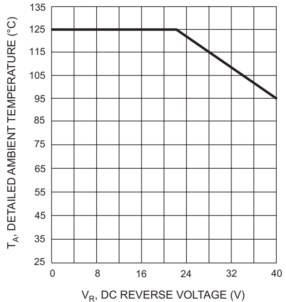
Fig. 4 Operating Temperature Derating
