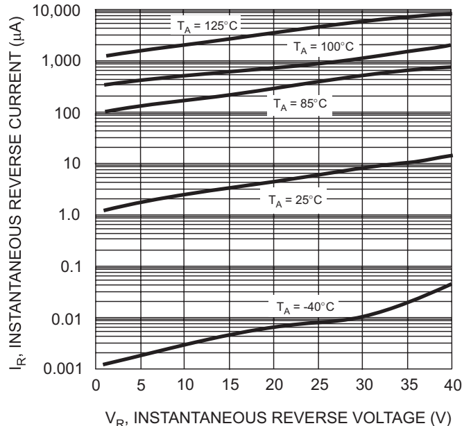
Fig. 2 Typical Pulsed Reverse Characteristics
