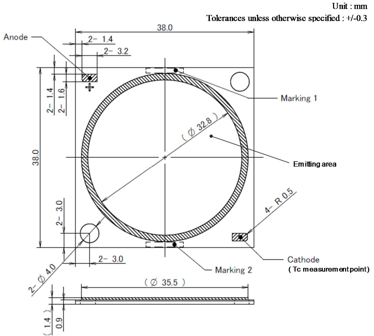
Figure 1. Outline drawing - Marking
