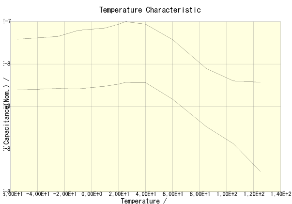
C1608X7R1E104K080AA(DC Bias = 0V) C1608X7R1E104K080AA(DC Bias = 12.5V)
