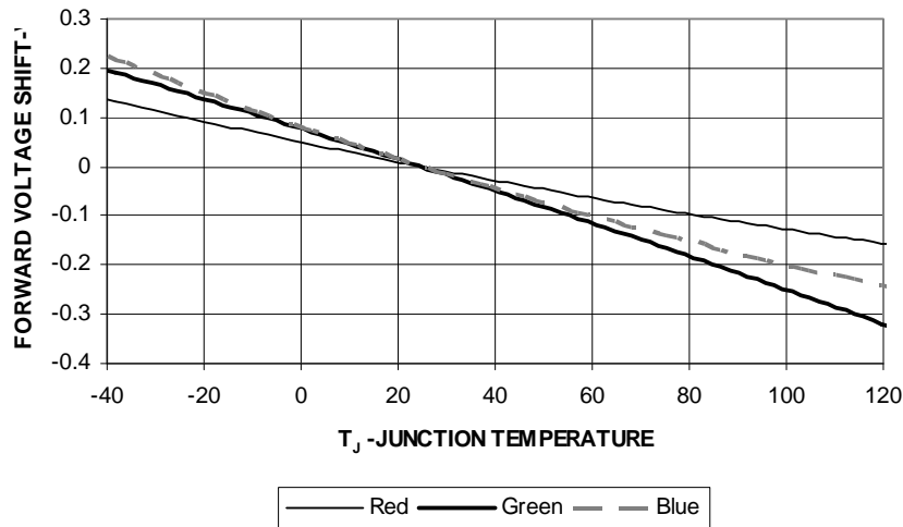
Figure 7: Relative Forward Voltage vs Junction Temperature
