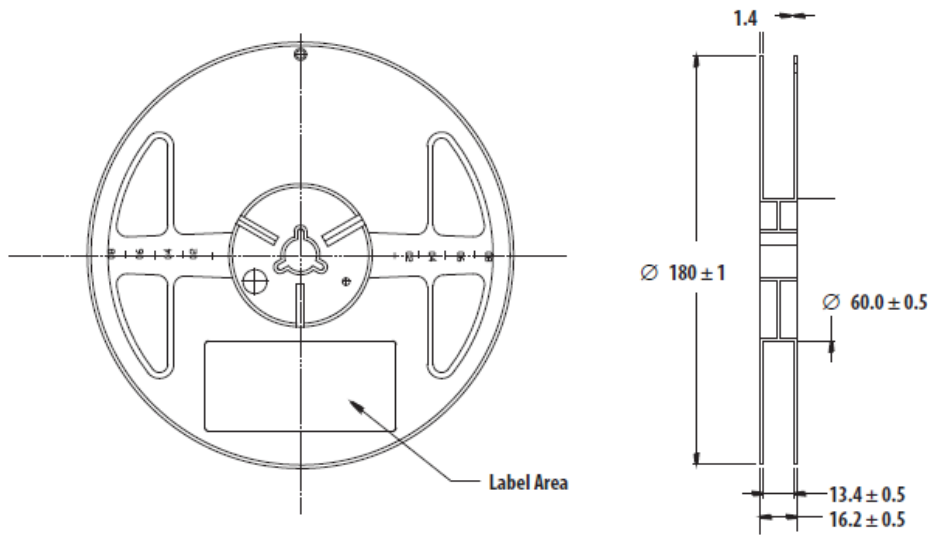
Figure 12. Reel Dimension
