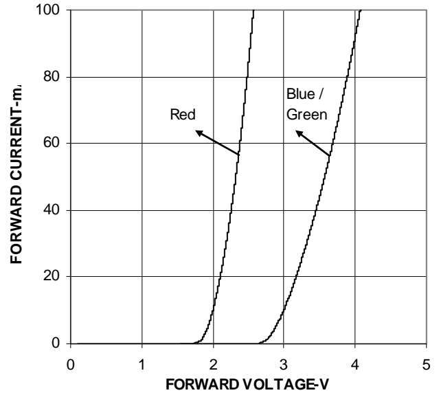
Figure 2: Forward Current-mA vs Forward Voltage-V
