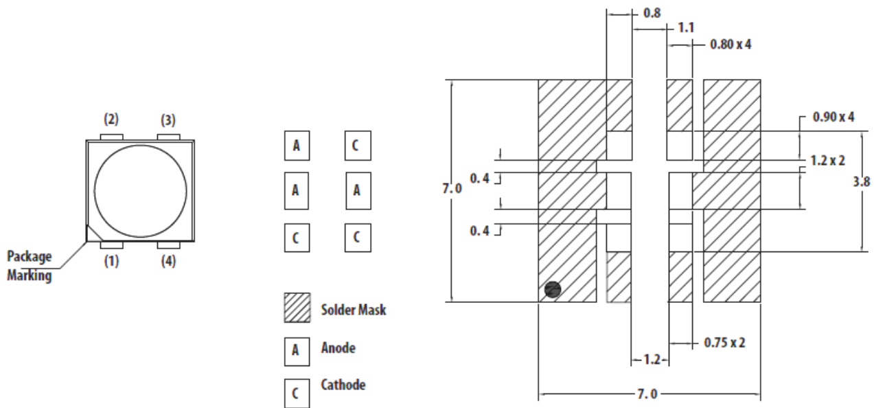
Figure 8. Recommended soldering land pattern.
