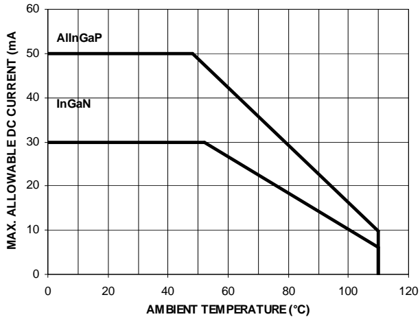
Figure 4a. Maximum forward current vs. ambient temperature. Derated based on T_{j,MAX} = 125^{\circ}C . (3 chips)
