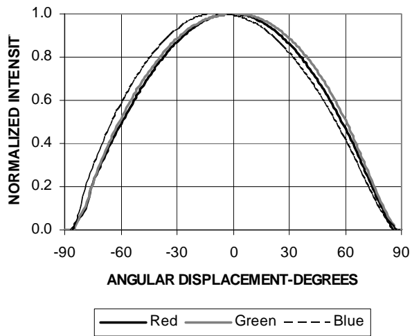
Figure 5: Radiation Pattern
