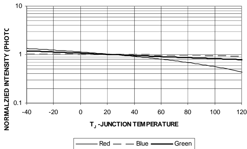
Figure 6: Relative Intensity vs Junction Temperature
