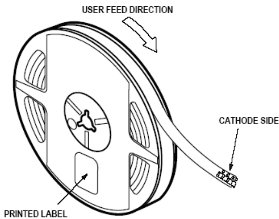
Figure 13. Reeling Orientation
