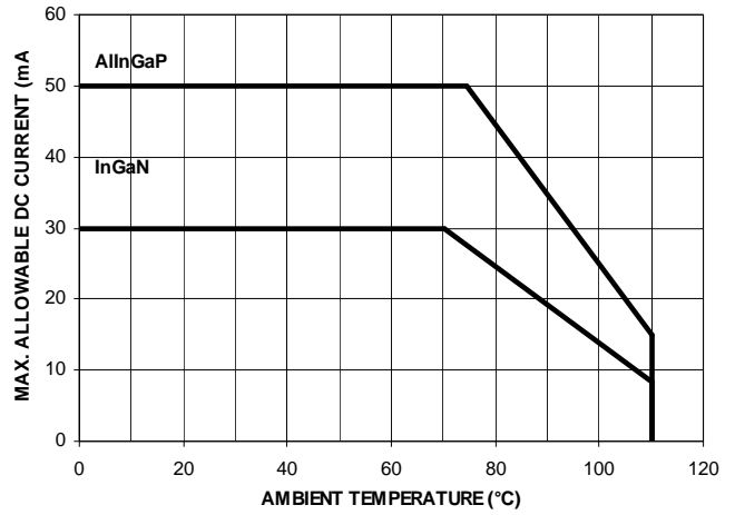
Figure 4b. Maximum forward current vs. ambient temperature. Derated based on T_{j,MAX} = 125^{\circ}C . (single chip)
