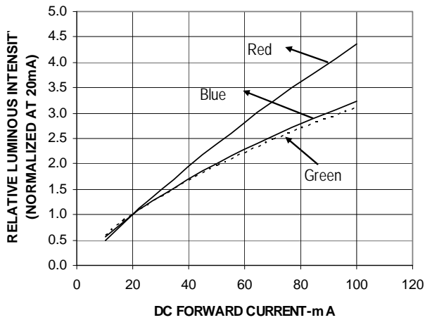
Figure 3: Relative Intensity vs Forward Current
