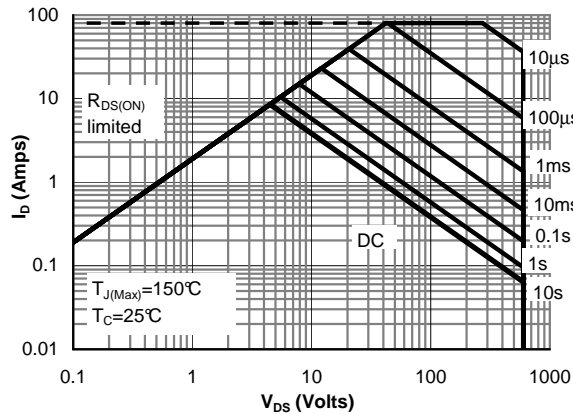
Figure 13: Maximum Forward Biased Safe Operating Area for AOTF20S60L(Note F)
