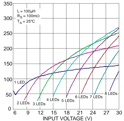
Fig. 27 Switching Frequency vs. Input Voltage
