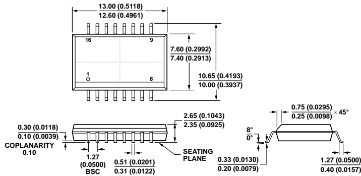
Figure 24. 16-Lead Standard Small Outline Package [SOIC_W] Wide Body (RW-16) Dimensions shown in millimeters and (inches)
