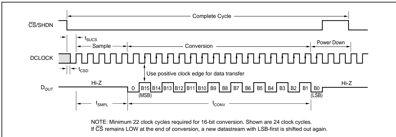
FIGURE 3. ADS8320 Basic Timing Diagrams.
