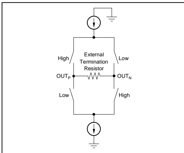
Figure 38. LVDS Buffer
