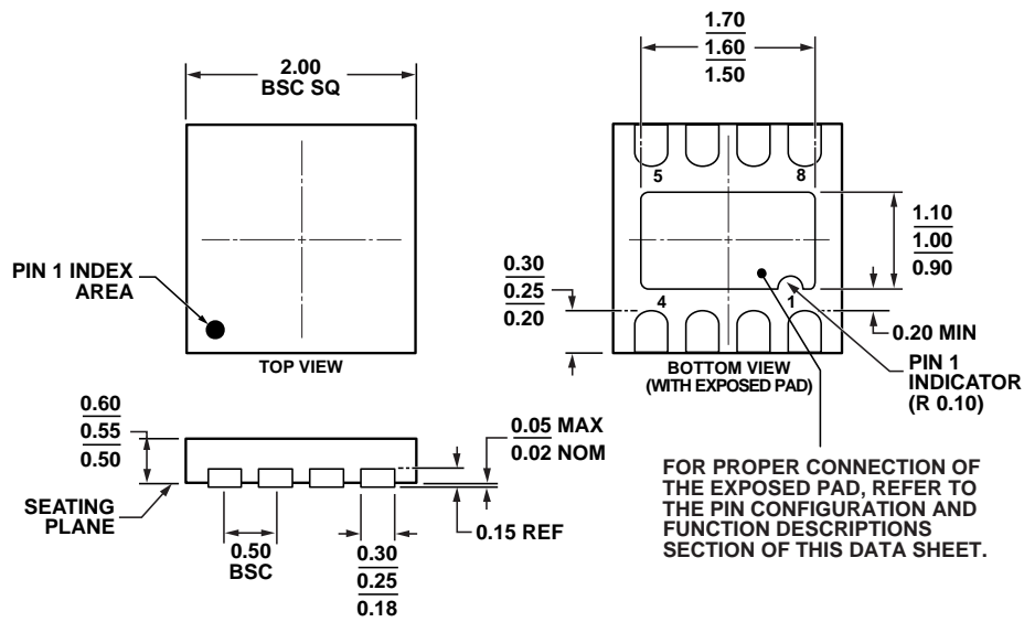
Figure 46. 8-Lead Lead Frame Chip Scale Package [LFCSP_UD] 2 mm x 2 mm Body, Ultra Thin, Dual Lead (CP-8-8) Dimensions shown in millimeters
