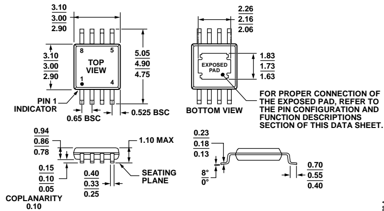
Figure 45. 8-Lead Mini Small Outline Package with Exposed Pad [MINI_SO_EP] (RH-8-1) Dimensions shown in millimeters
