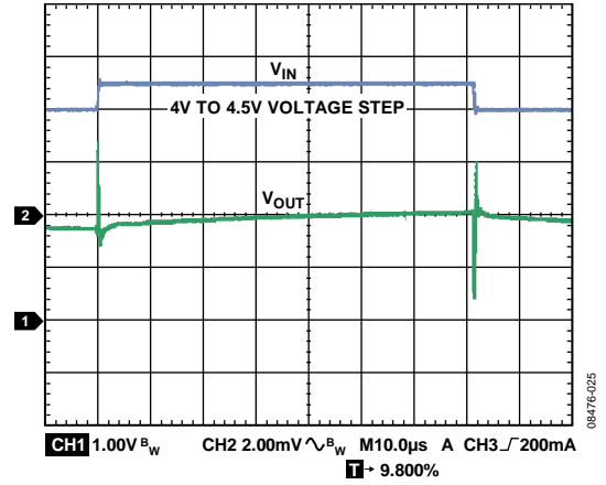
Figure 27. Line Transient Response, Load Current = 500 mA
