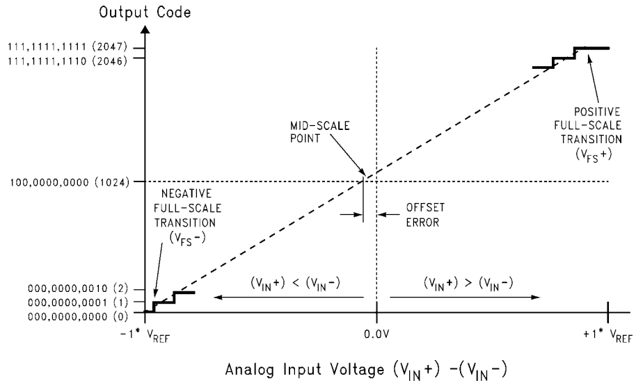
FIGURE 1. Transfer Characteristic (Offset Binary Format)
