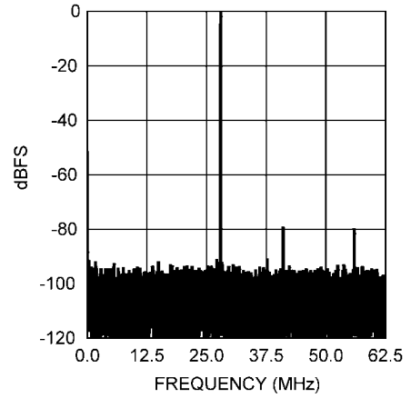
Spectral Response @ 278 MHz Input
