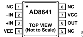
NC = NO CONNECT Figure 2. 8-Lead SOIC (R-8)
