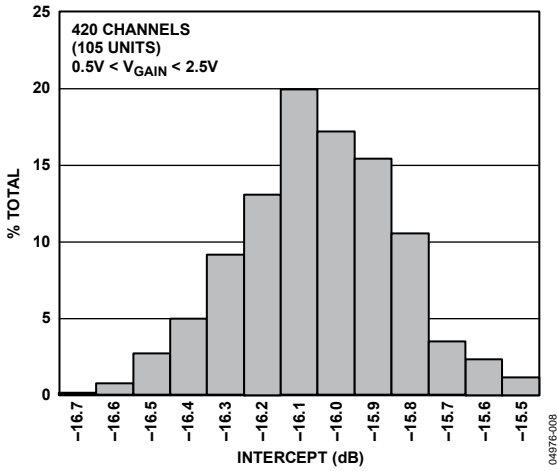
Figure 9. Intercept Histogram
