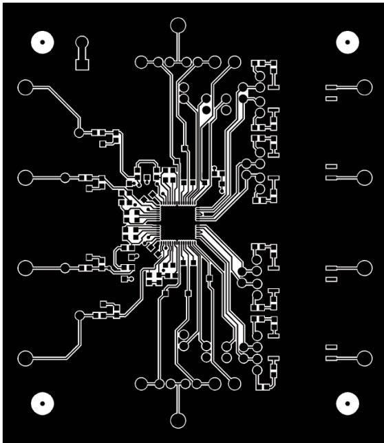
Figure 64. AD8335-EVALZ Component Side Copper
