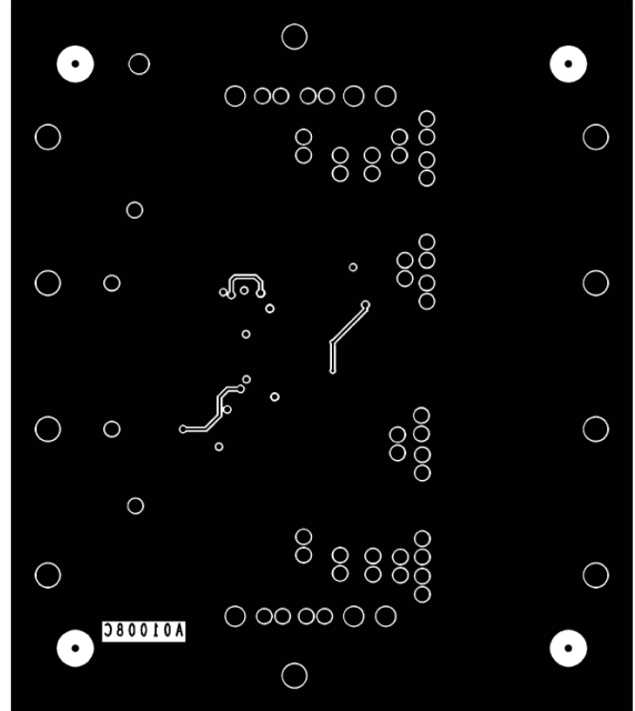
Figure 65. AD8335-EVALZ Secondary Side Copper
