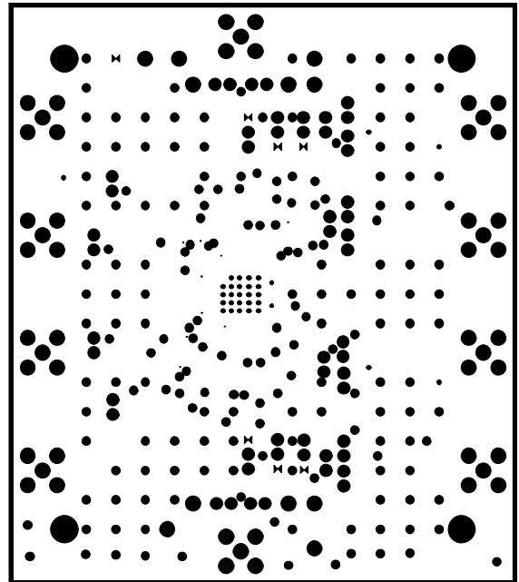
Figure 66. AD8335-EVALZ Internal Power Plane
