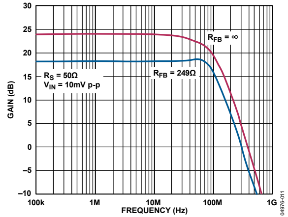
Figure 12. Frequency Response for a Terminated and Underterminated 50\ \Omega Source (See Figure 49)
