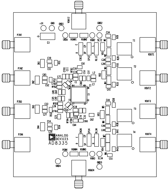
Figure 63. AD8335-EVALZ Assembly
