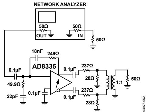
Figure 52. Test Circuit for S11 Measurements
