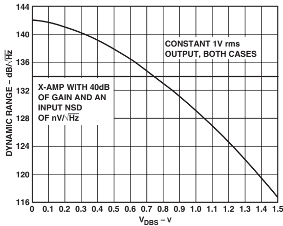
Figure 11. Dynamic Range in \text{dB}/\sqrt{\text{Hz}} vs. V_{DBS} ( V_{MAG} = 0.5\text{ V} , 1\text{ V rms} output) Compared with a Representative X-AMP (Simulation)
