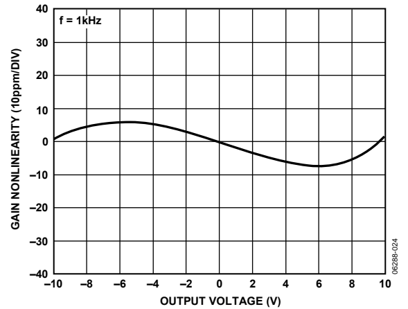
Figure 23. Gain Nonlinearity vs. Output Voltage, G = 1 , R_L = 10\text{ k}\Omega, 2\text{ k}\Omega, 600\ \Omega
