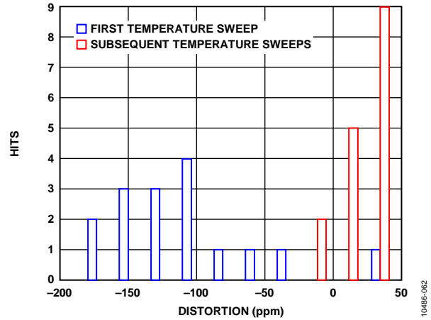
Figure 55. Thermal Hysteresis
