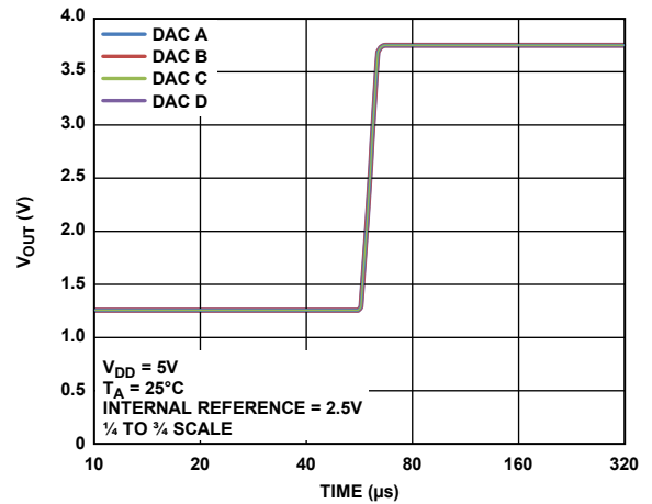
Figure 34. Settling Time, 5.25 V
