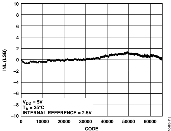
Figure 13. AD5696R INL
