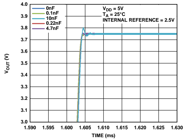
Figure 44. Settling Time vs. Capacitive Load
