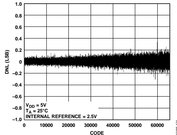
Figure 16. AD5696R DNL
