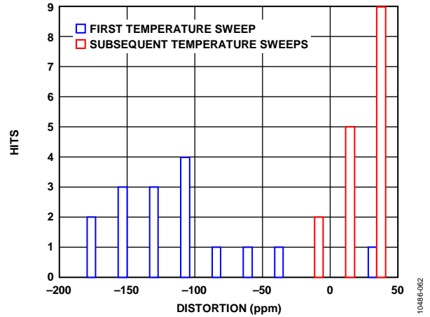
Figure 57. Thermal Hysteresis
