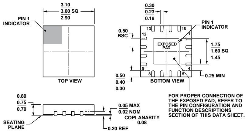
Figure 61. 16-Lead Lead Frame Chip Scale Package [LFCSP_WQ] 3 mm x 3 mm Body, Very Very Thin Quad (CP-16-22)
