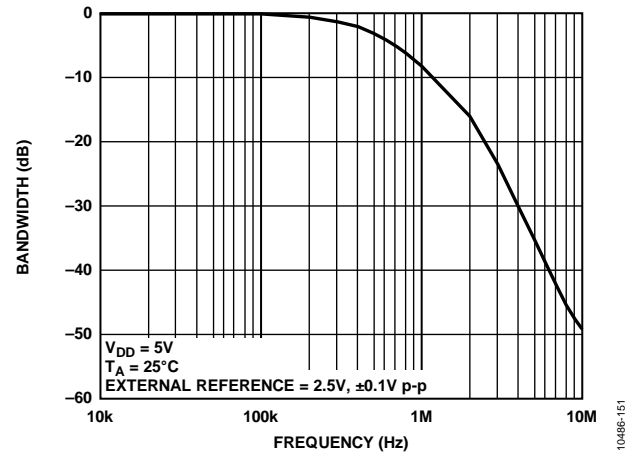
Figure 45. Multiplying Bandwidth, External Reference = 2.5 V, \pm 0.1 V p-p, 10 kHz to 10 MHz
