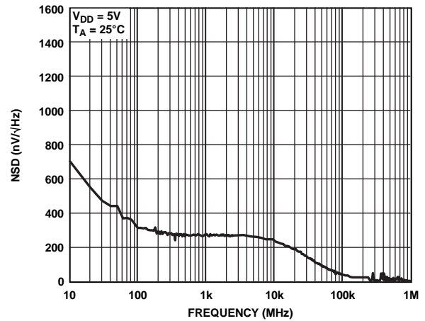
Figure 12. Internal Reference Noise Spectral Density vs. Frequency
