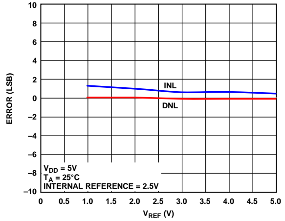
Figure 23. INL Error and DNL Error vs. V_{REF}
