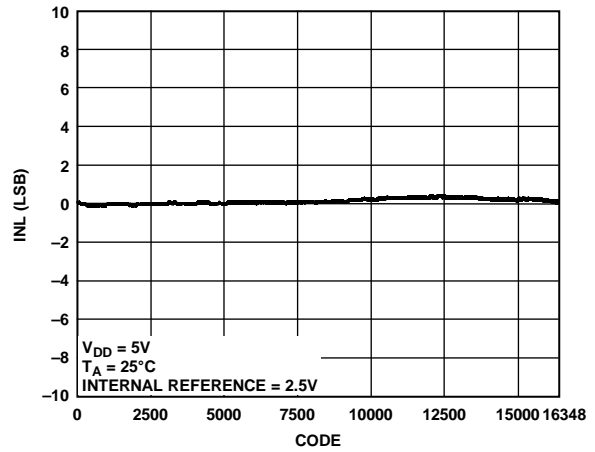
Figure 17. AD5685R INL
