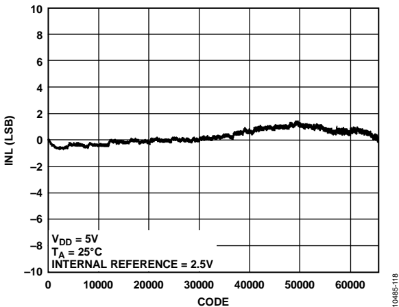
Figure 16. AD5686R INL
