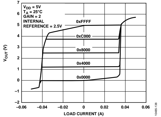
Figure 35. Source and Sink Capability at 5 V
