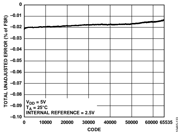
Figure 31. TUE vs. Code
