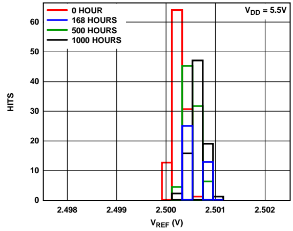
Figure 11. Reference Long-Term Stability/Drift
