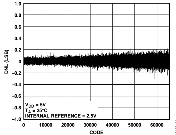
Figure 19. AD5686R DNL
