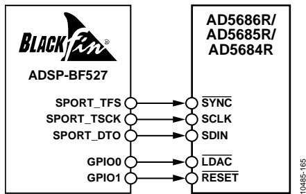
Figure 61. SPORT Interface
