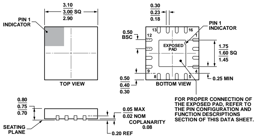
Figure 64. 16-Lead Lead Frame Chip Scale Package [LFCSP_WQ] 3 mm x 3 mm Body, Very Very Thin Quad (CP-16-22)
