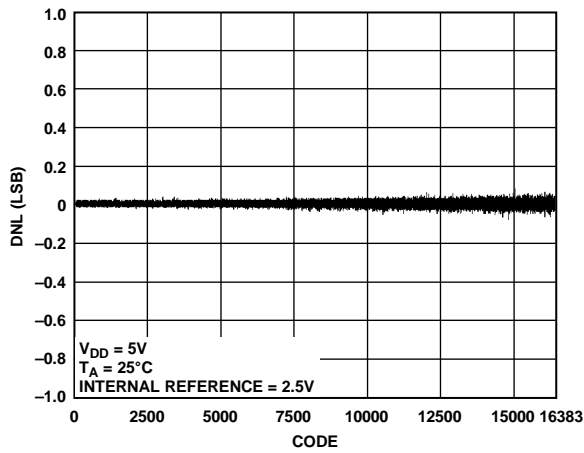
Figure 20. AD5685R DNL
