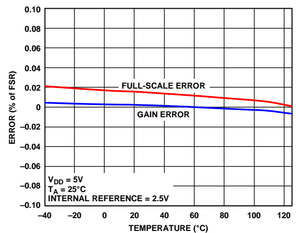
Figure 25. Gain Error and Full-Scale Error vs. Temperature
