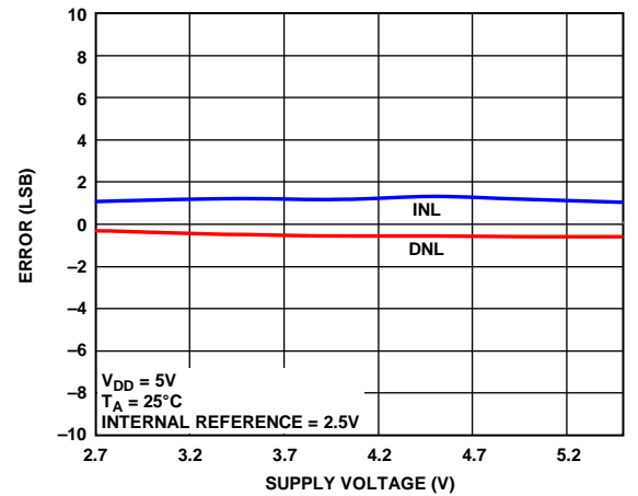
Figure 24. INL Error and DNL Error vs. Supply Voltage
