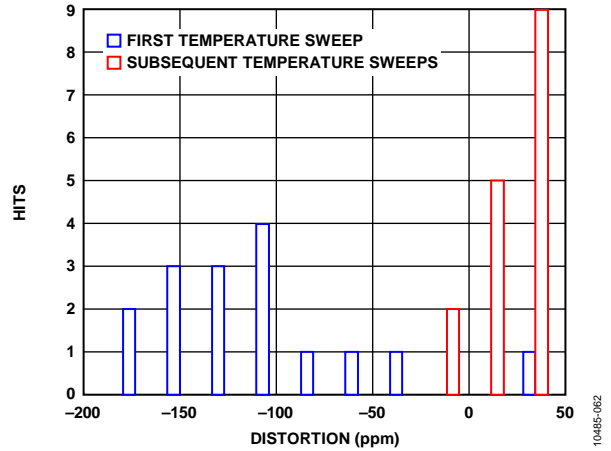
Figure 59. Thermal Hysteresis
