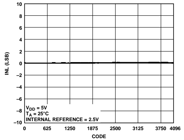
Figure 18. AD5684R INL
