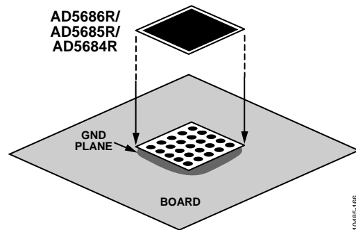
Figure 62. Paddle Connection to Board
