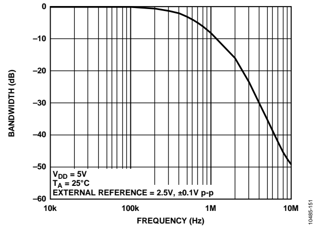
Figure 48. Multiplying Bandwidth, External Reference = 2.5 V, ±0.1 V p-p, 10 kHz to 10 MHz
