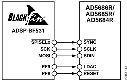
Figure 60. ADSP-BF531 Interface
