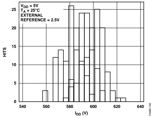
Figure 32. I_{DD} Histogram with External Reference, 5 V
