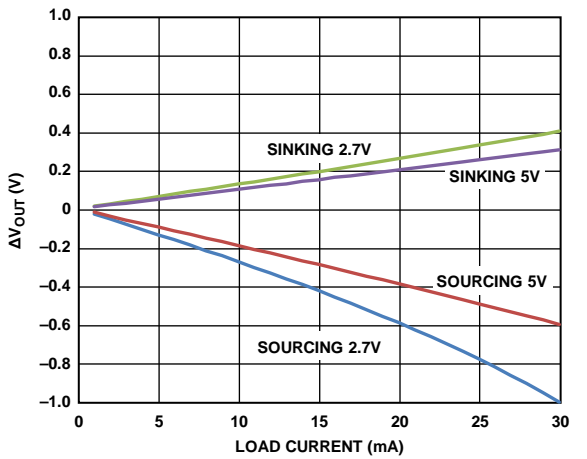
Figure 34. Headroom/Footroom vs. Load Current
