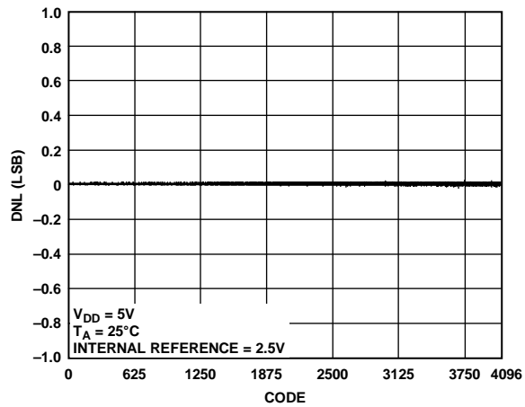
Figure 21. AD5684R DNL
