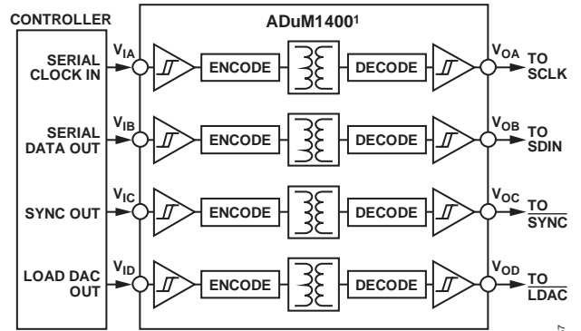
Figure 63. Isolated Interface
