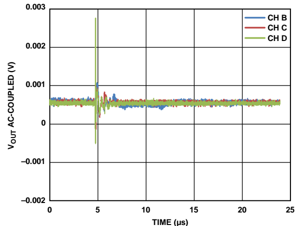
Figure 42. Analog Crosstalk, Channel A
