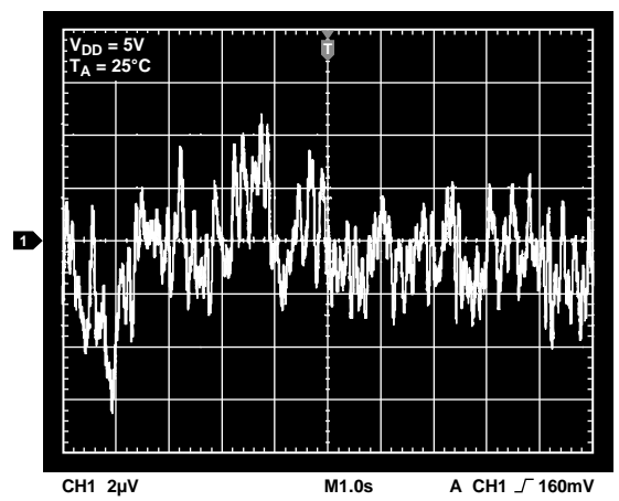
Figure 13. Internal Reference Noise, 0.1 Hz to 10 Hz
