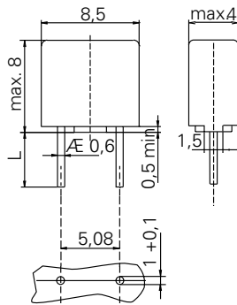
Holes in PCB Long Leads (L=18.8mm) Short Leads (L=4.3mm)
