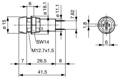
Variants 3101.0010 and 3101.0210
