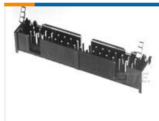
TE Model / Part #2-1761606-3 IDC LOW PRO HDR 10P VERT LG LAT BLUE
