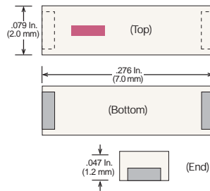
Case 43-1
