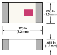
Case 18-4
