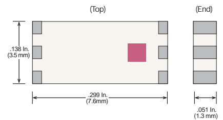
Case 44-1
