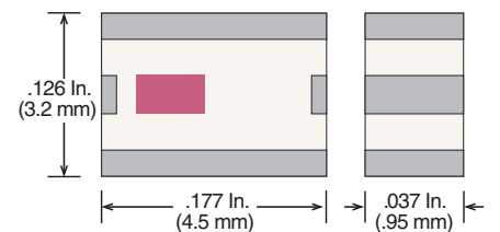
Case 44-1
